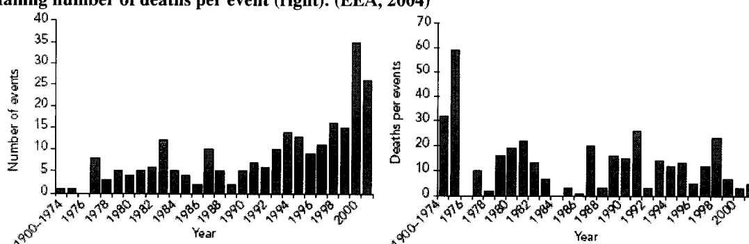
Figure 3.3: the increasing number of flood events in Europe over time (left), contrasted to the falling number of deaths per event (right). (EEA, 2004)
