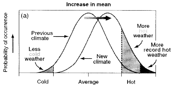
Figure 2.3: a warming shift in the average Temperature (IPCC, 2001)
